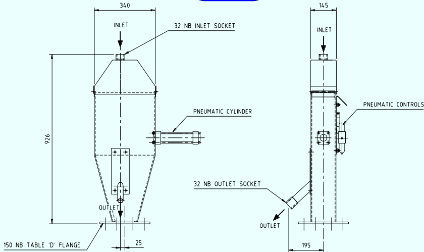
TYPICAL ARRANGEMENT OF SINGLE SLURRY SAMPLER
