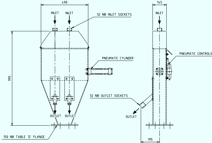
TYPICAL ARRANGEMENT OF DUAL SLURRY SAMPLER
